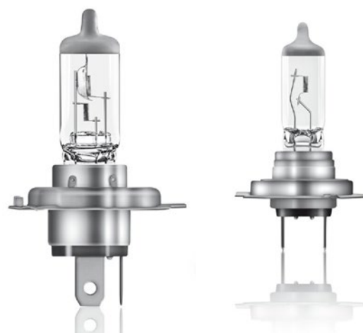
Original Line Autolamp H4 12V 60/55W Ampoule Original Line H4 12V 60/55W
